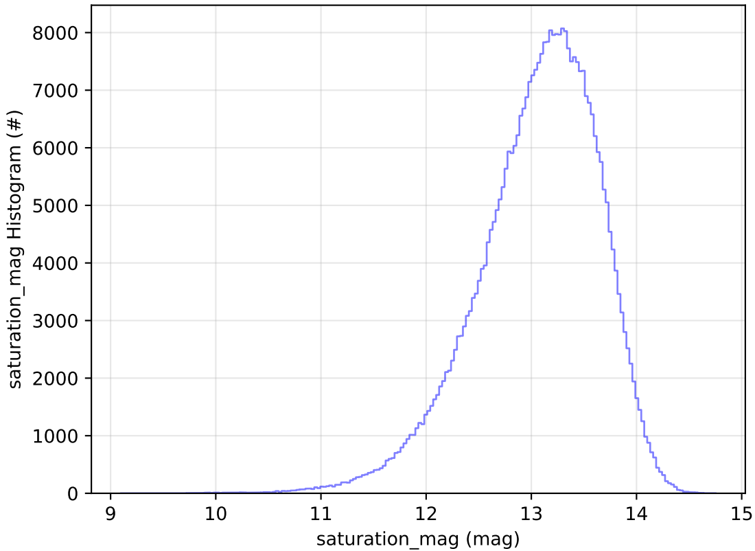
too_elab_r256_d3_griz_v3.4_10yrs WFD y band: saturation_mag Histogram
