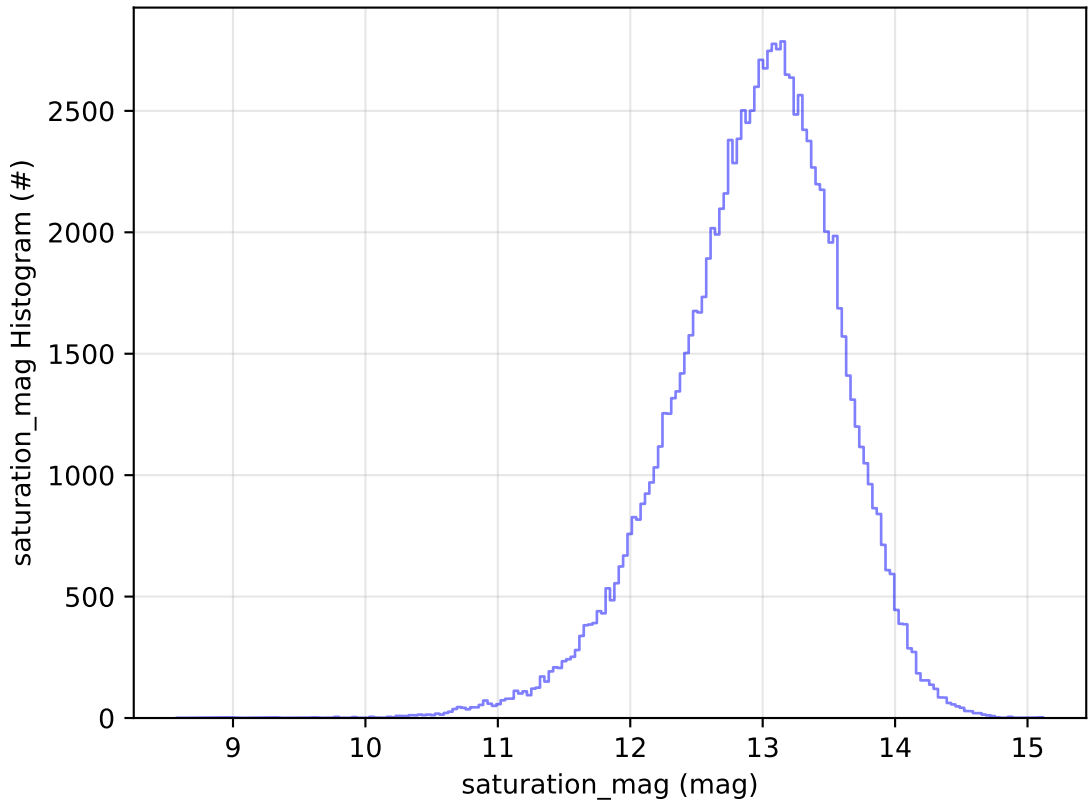
too_elab_r256_d3_griz_v3.4_10yrs WFD u band: saturation_mag Histogram
