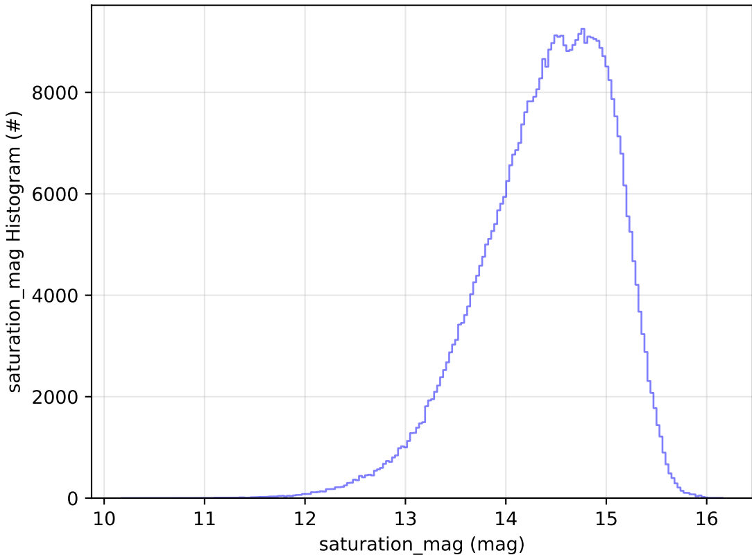
too_elab_r256_d3_griz_v3.4_10yrs WFD i band: saturation_mag Histogram
