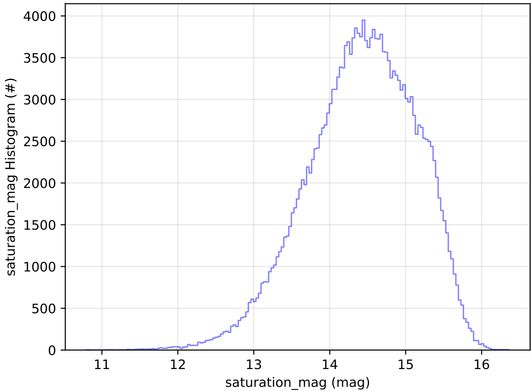
too_elab_r256_d3_griz_v3.4_10yrs WFD g band: saturation_mag Histogram
