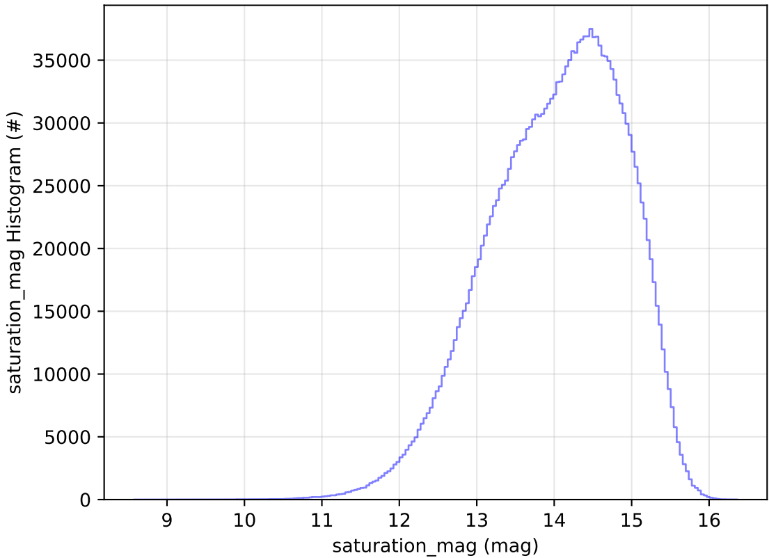
too_elab_r256_d3_griz_v3.4_10yrs WFD all bands: saturation_mag Histogram
