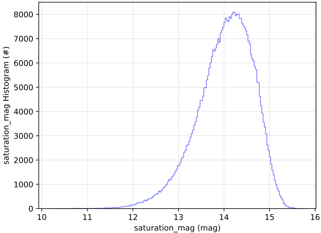
too_elab_r256_d3_griz_v3.4_10yrs All sky z band: saturation_mag Histogram
