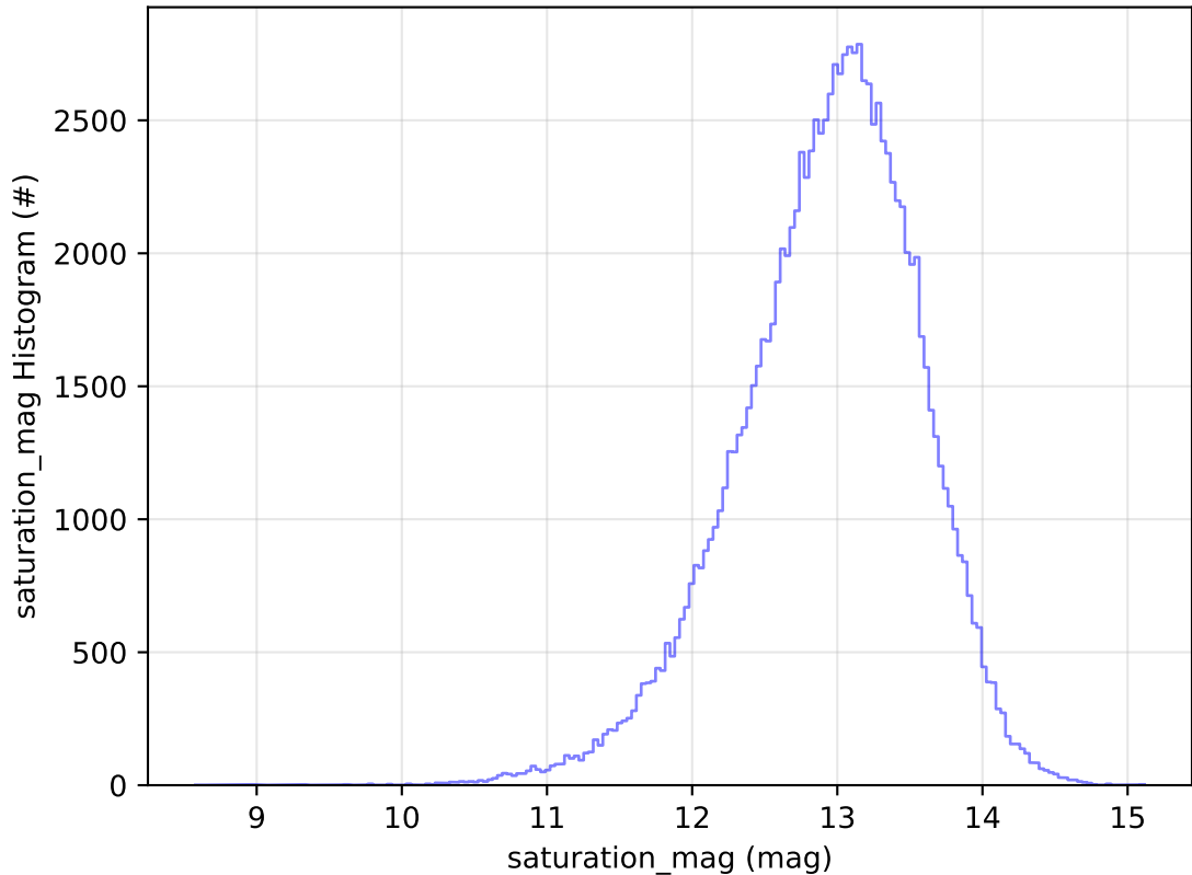
too_elab_r256_d3_griz_v3.4_10yrs All sky u band: saturation_mag Histogram
