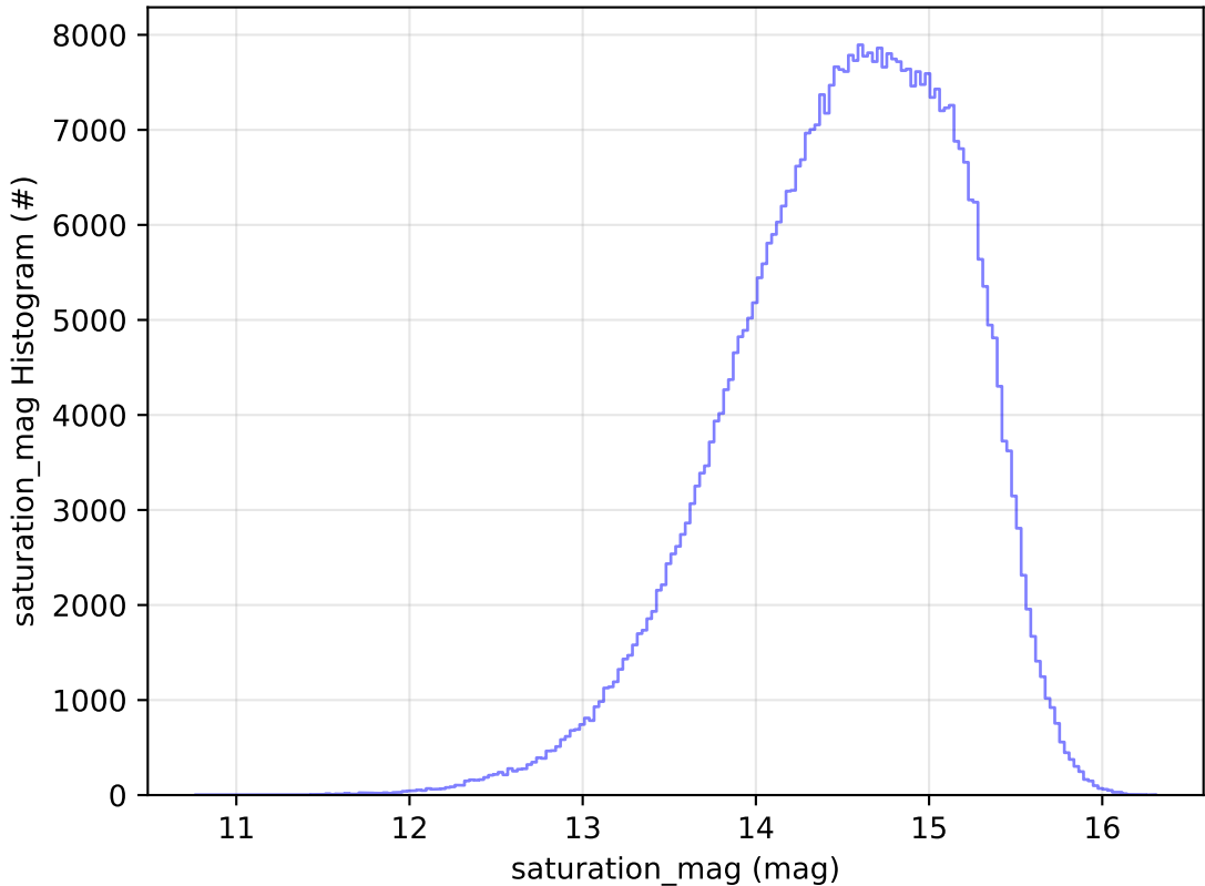
too_elab_r256_d3_griz_v3.4_10yrs All sky r band: saturation_mag Histogram
