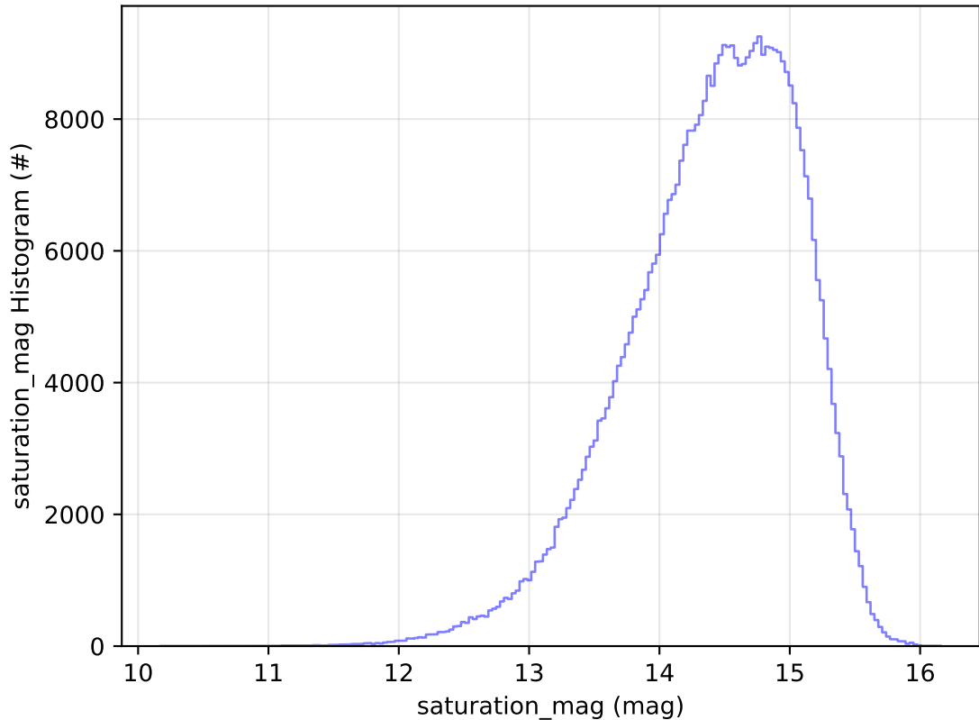
too_elab_r256_d3_griz_v3.4_10yrs All sky i band: saturation_mag Histogram
