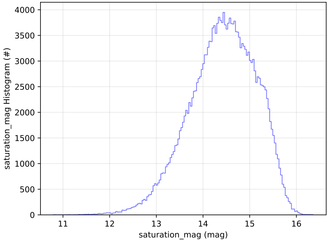
too_elab_r256_d3_griz_v3.4_10yrs All sky g band: saturation_mag Histogram
