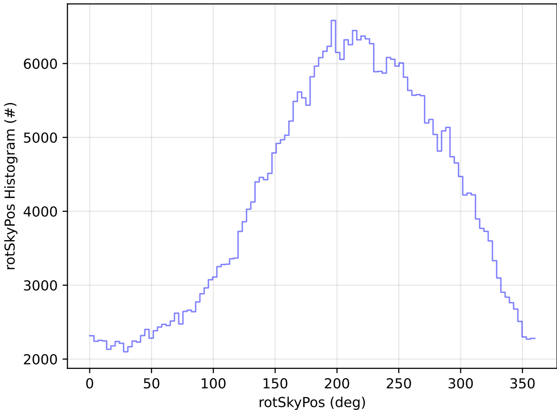
too_elab_r256_d3_griz_v3.4_10yrs WFD z band: rotSkyPos Histogram
