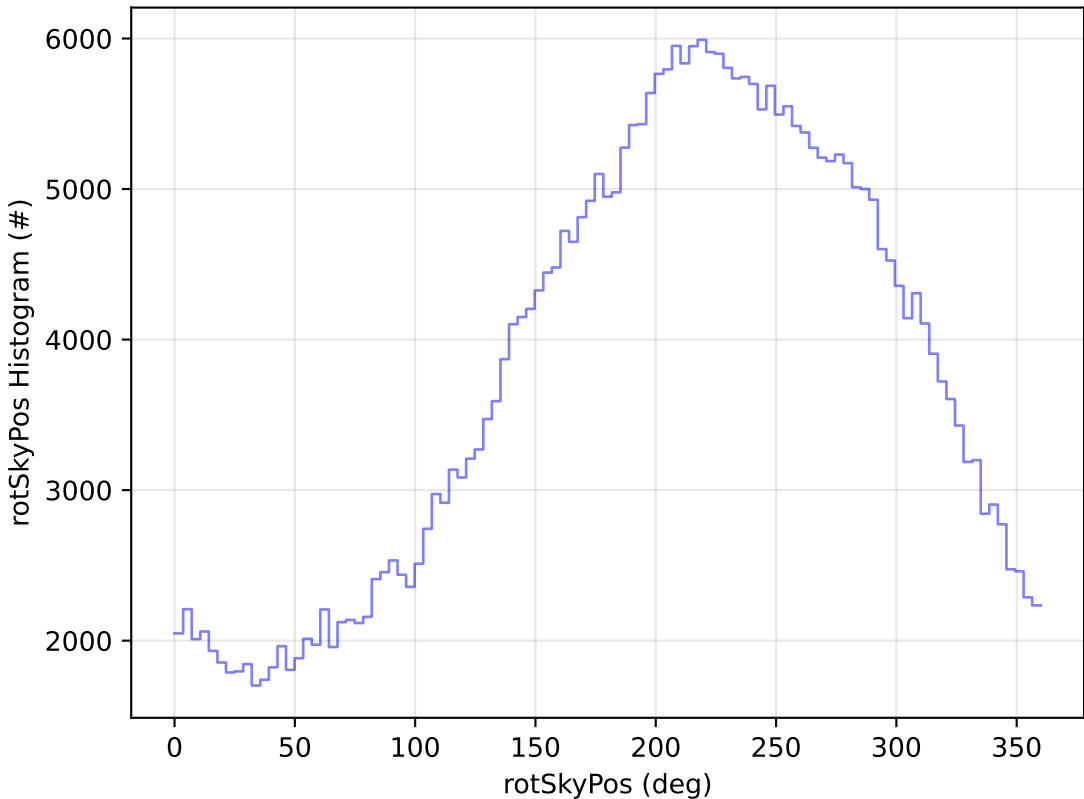
too_elab_r256_d3_griz_v3.4_10yrs WFD y band: rotSkyPos Histogram
