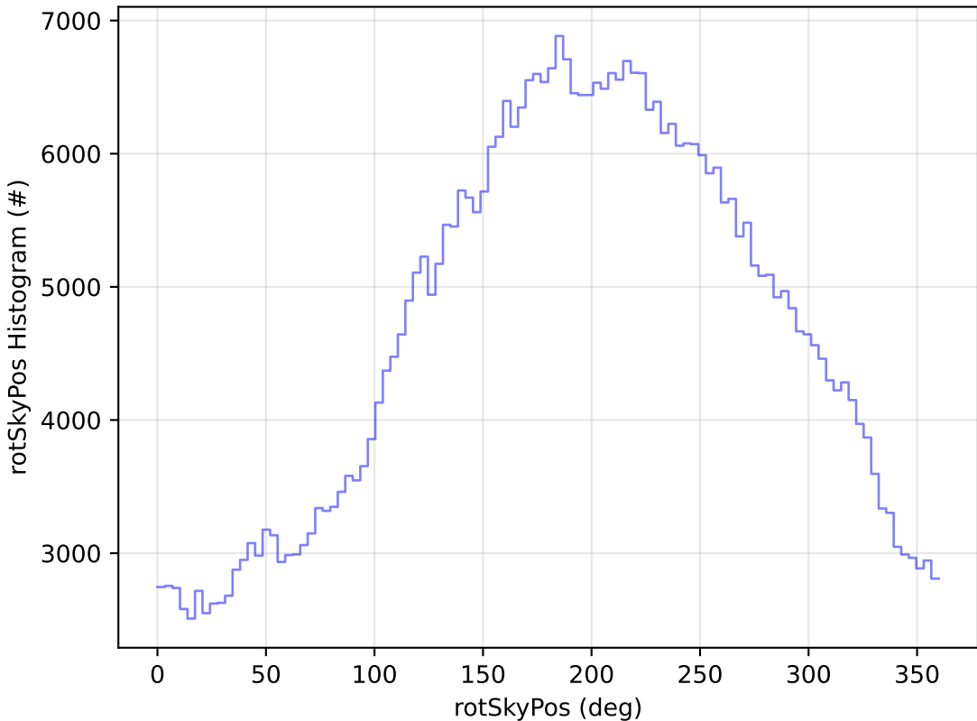
too_elab_r256_d3_griz_v3.4_10yrs WFD r band: rotSkyPos Histogram
