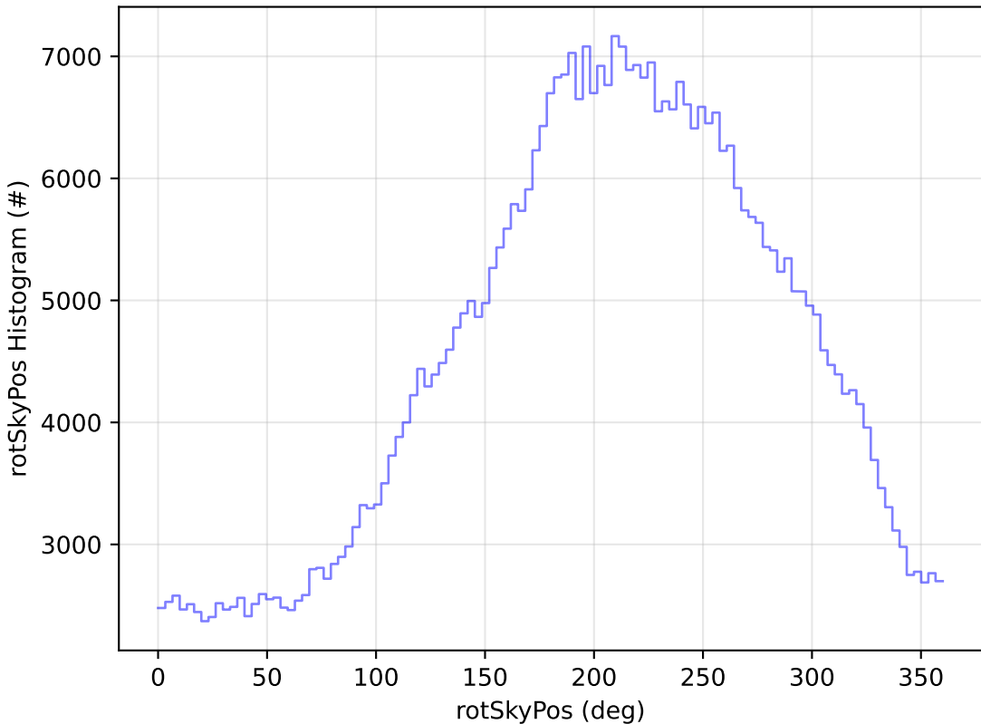
too_elab_r256_d3_griz_v3.4_10yrs WFD i band: rotSkyPos Histogram
