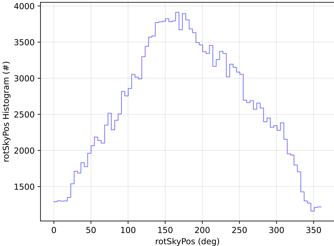
too_elab_r256_d3_griz_v3.4_10yrs WFD g band: rotSkyPos Histogram
