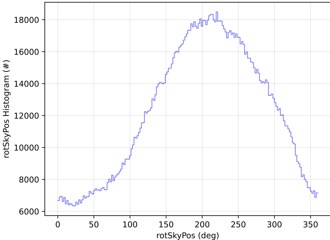
too_elab_r256_d3_griz_v3.4_10yrs WFD all bands: rotSkyPos Histogram
