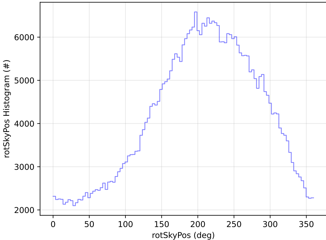
too_elab_r256_d3_griz_v3.4_10yrs All sky z band: rotSkyPos Histogram
