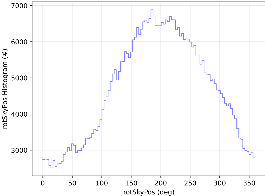
too_elab_r256_d3_griz_v3.4_10yrs All sky r band: rotSkyPos Histogram
