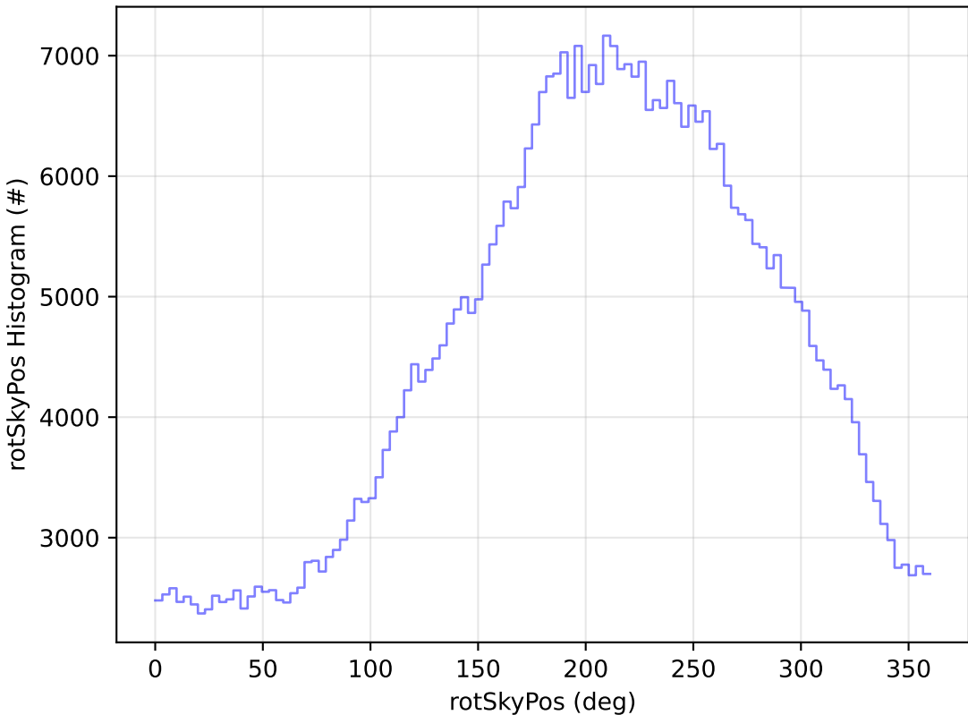
too_elab_r256_d3_griz_v3.4_10yrs All sky i band: rotSkyPos Histogram
