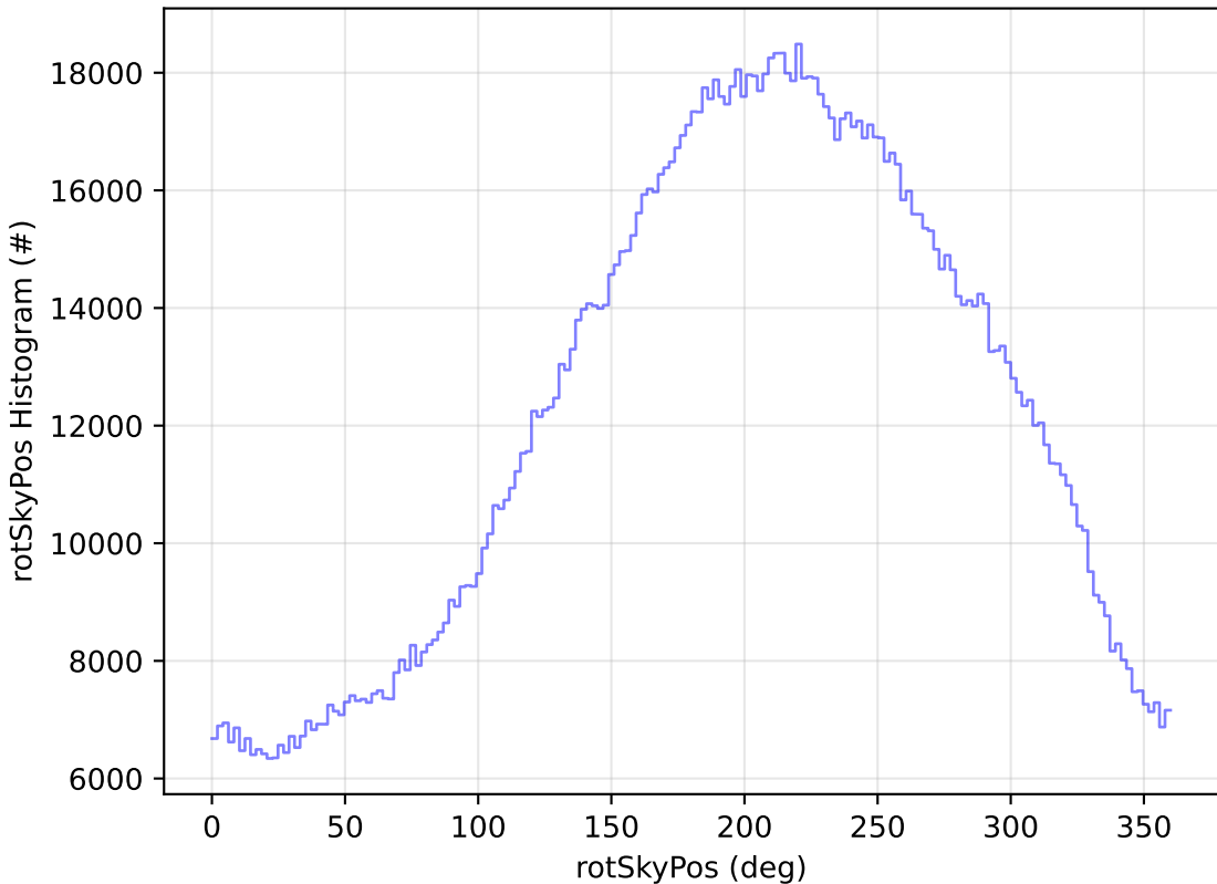
too_elab_r256_d3_griz_v3.4_10yrs All sky all bands: rotSkyPos Histogram
