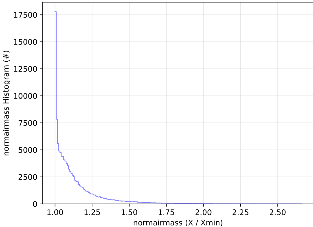
too_elab_r256_d3_griz_v3.4_10yrs WFD u band: normairmass Histogram
