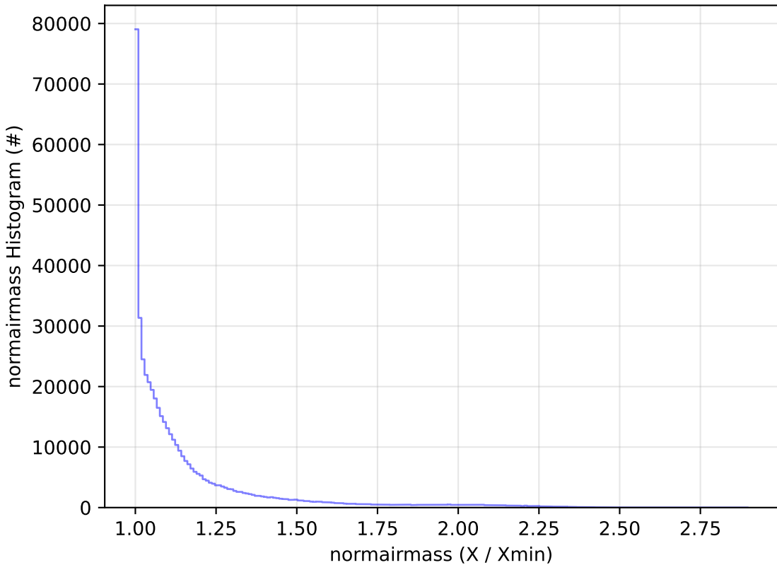
too_elab_r256_d3_griz_v3.4_10yrs WFD r band: normairmass Histogram
