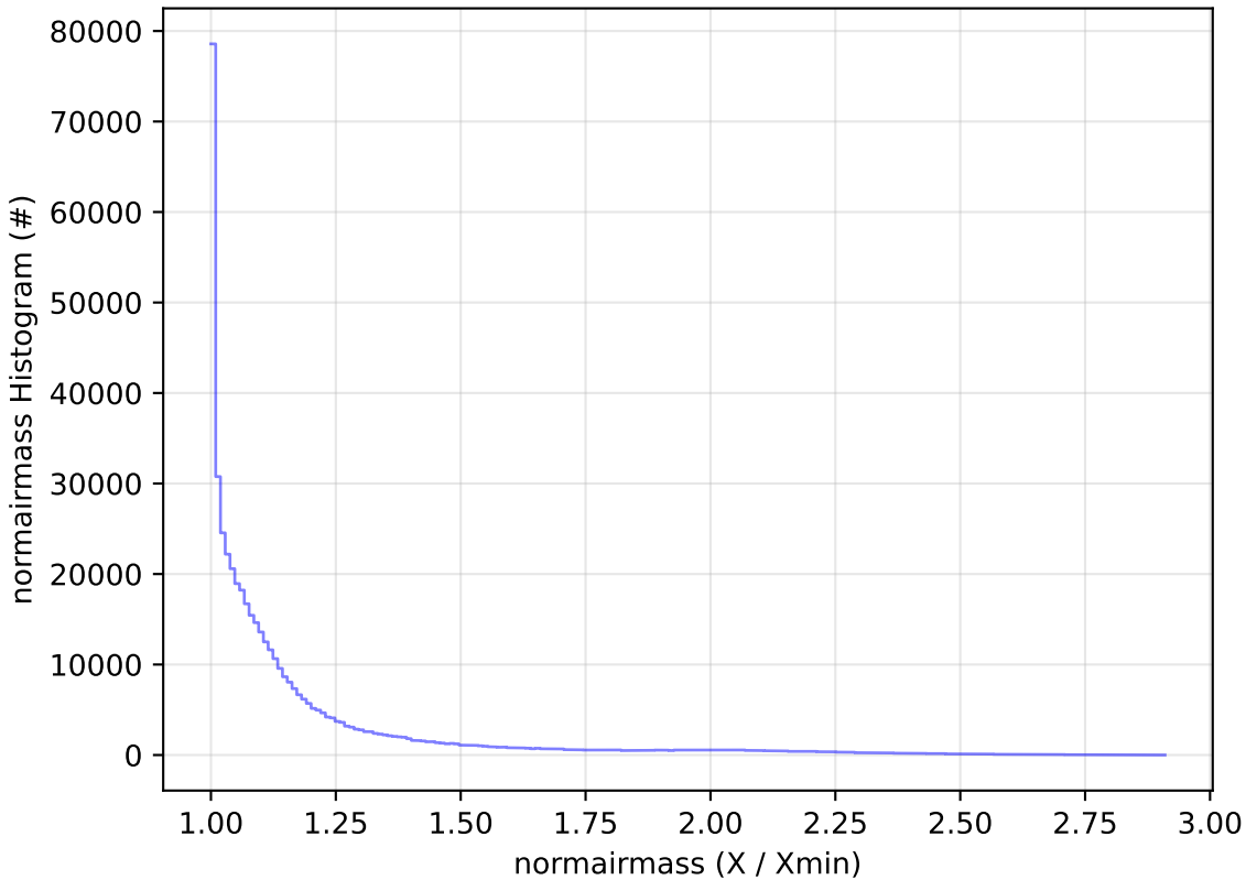
too_elab_r256_d3_griz_v3.4_10yrs WFD i band: normairmass Histogram
