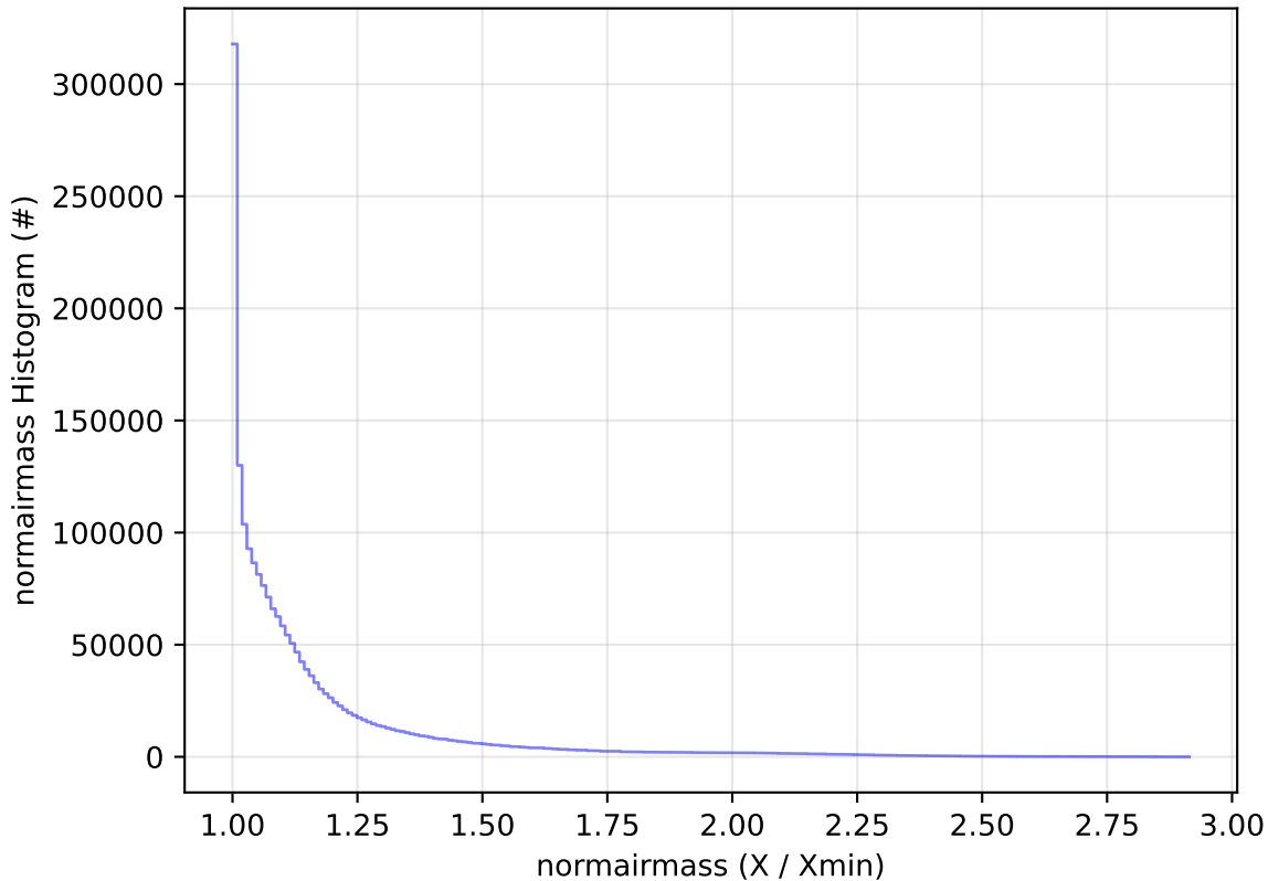
too_elab_r256_d3_griz_v3.4_10yrs WFD all bands: normairmass Histogram
