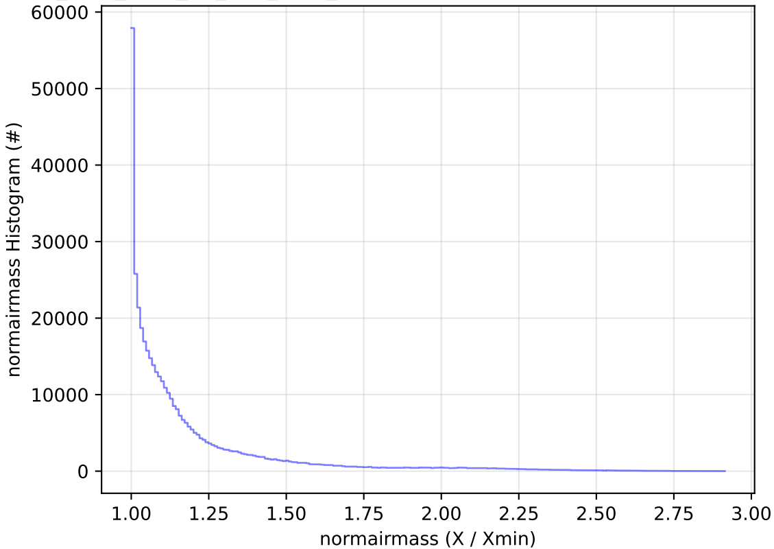
too_elab_r256_d3_griz_v3.4_10yrs All sky z band: normairmass Histogram
