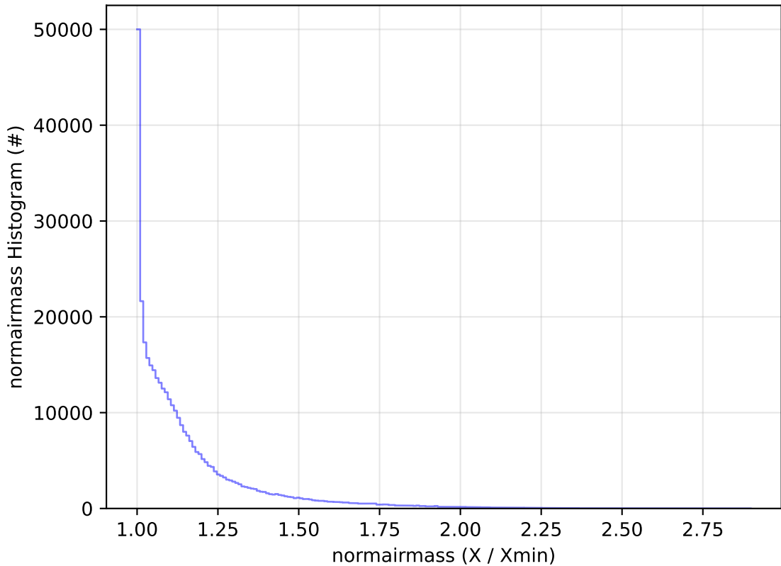
too_elab_r256_d3_griz_v3.4_10yrs All sky y band: normairmass Histogram
