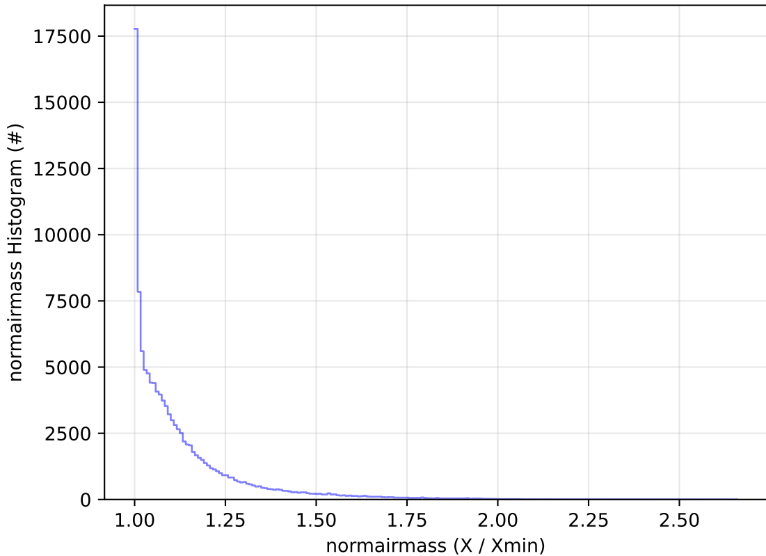
too_elab_r256_d3_griz_v3.4_10yrs All sky u band: normairmass Histogram
