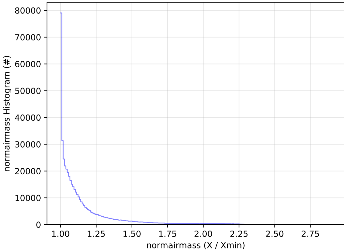
too_elab_r256_d3_griz_v3.4_10yrs All sky r band: normairmass Histogram
