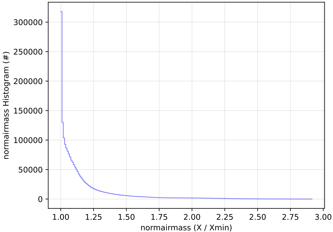
too_elab_r256_d3_griz_v3.4_10yrs All sky all bands: normairmass Histogram
