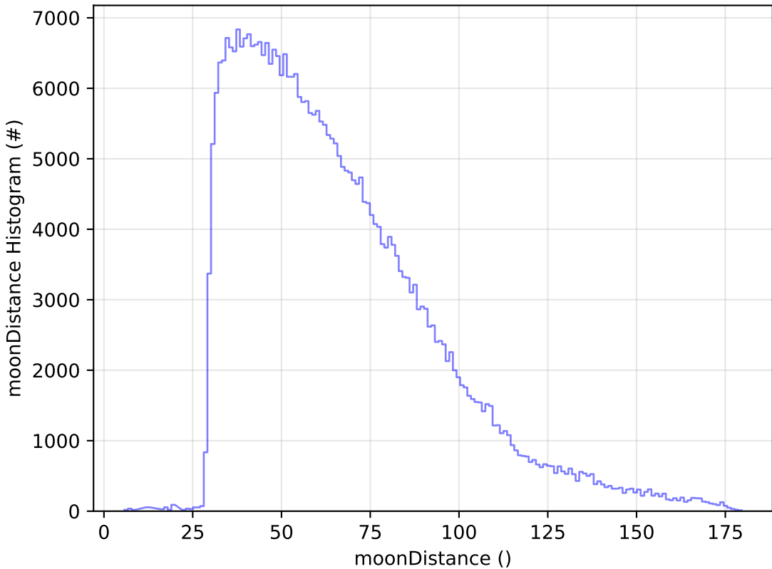
too_elab_r256_d3_griz_v3.4_10yrs WFD y band: moonDistance Histogram
