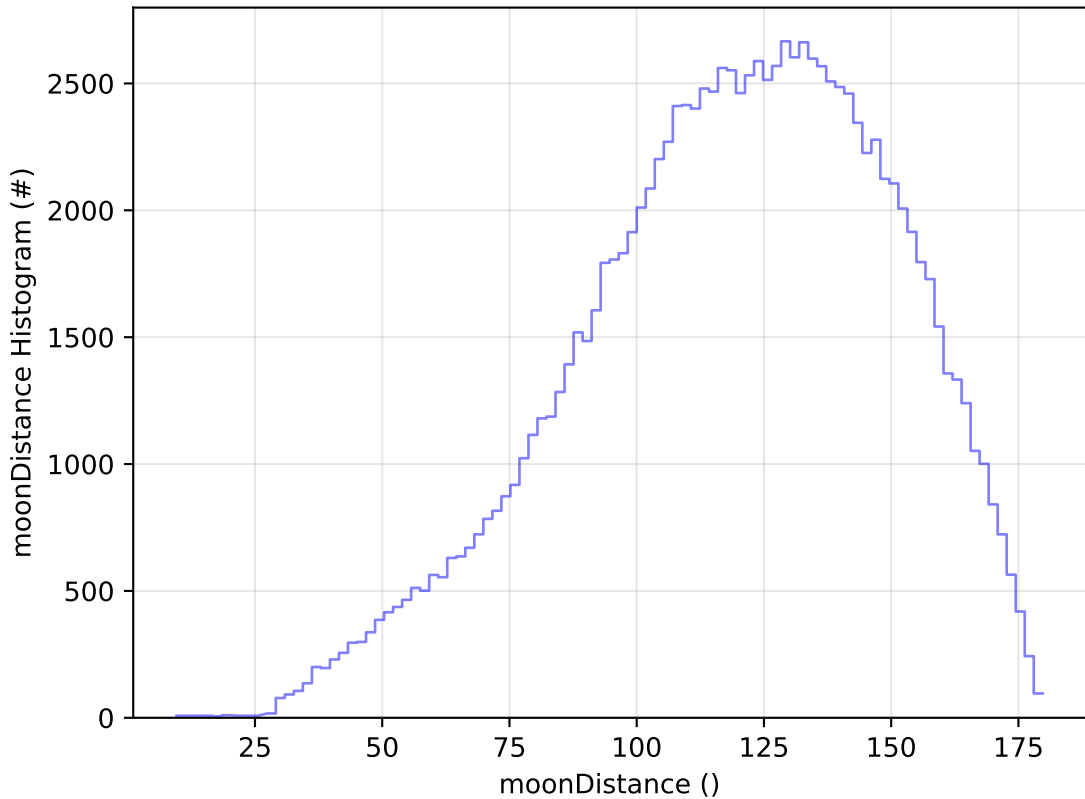
too_elab_r256_d3_griz_v3.4_10yrs WFD u band: moonDistance Histogram
