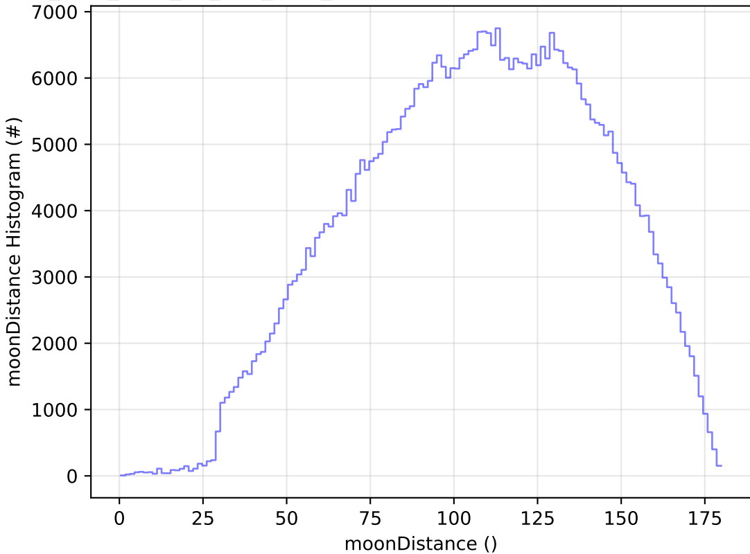
too_elab_r256_d3_griz_v3.4_10yrs WFD r band: moonDistance Histogram
