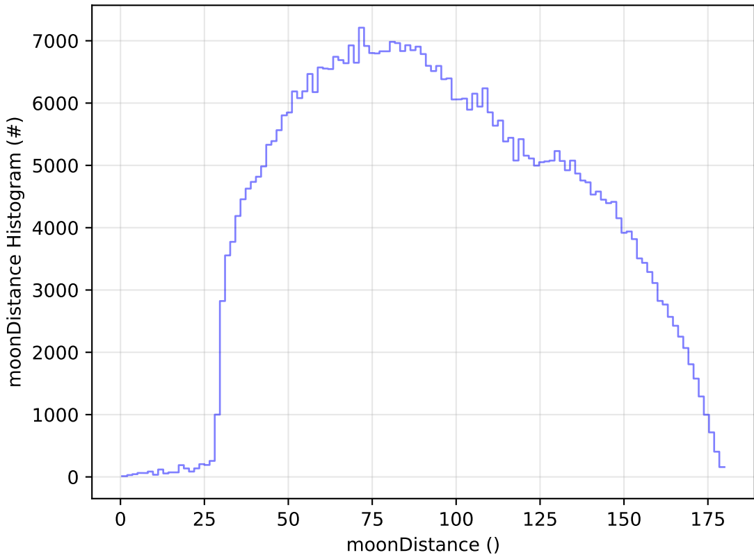
too_elab_r256_d3_griz_v3.4_10yrs WFD i band: moonDistance Histogram
