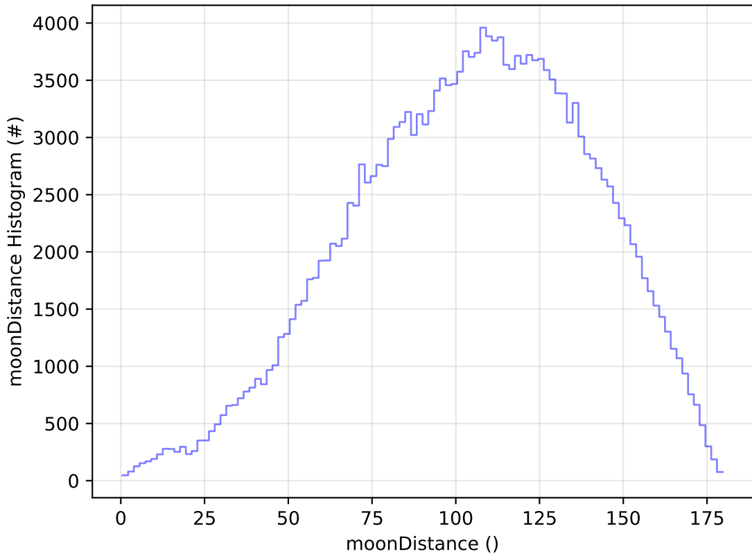
too_elab_r256_d3_griz_v3.4_10yrs WFD g band: moonDistance Histogram
