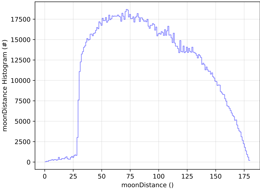
too_elab_r256_d3_griz_v3.4_10yrs WFD all bands: moonDistance Histogram
