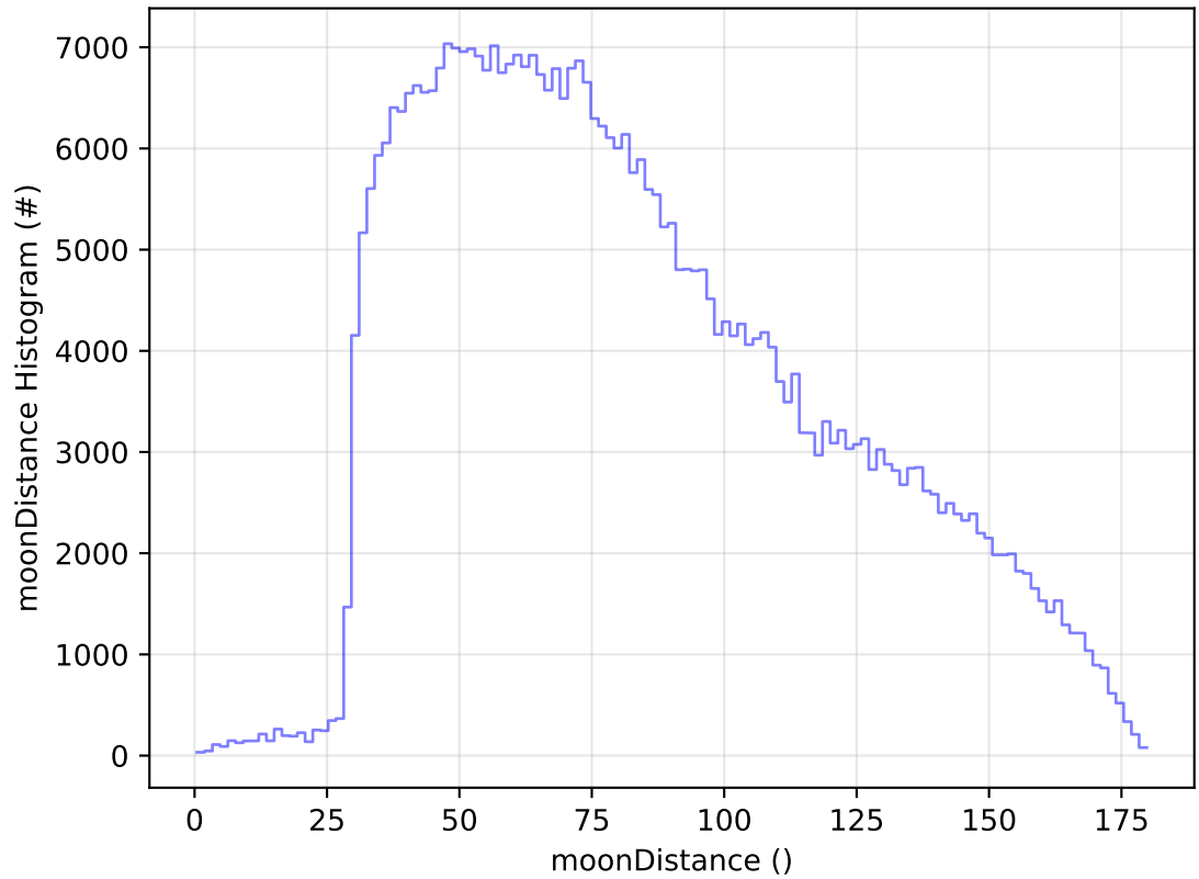
too_elab_r256_d3_griz_v3.4_10yrs All sky z band: moonDistance Histogram
