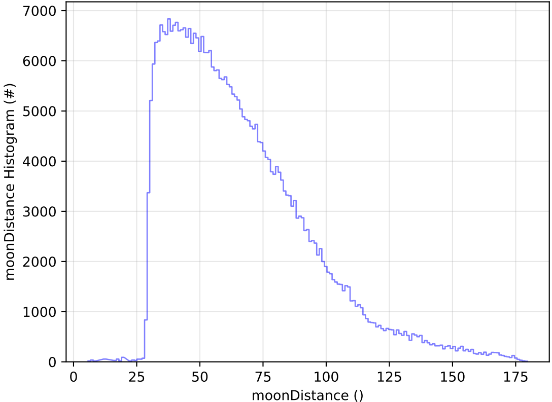
too_elab_r256_d3_griz_v3.4_10yrs All sky y band: moonDistance Histogram
