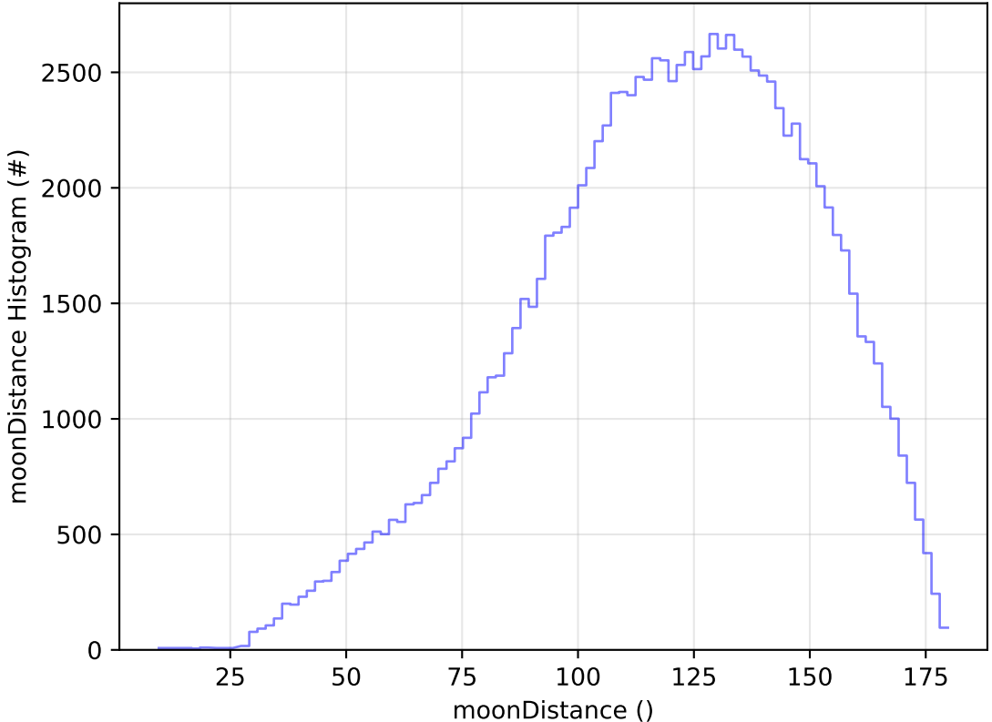
too_elab_r256_d3_griz_v3.4_10yrs All sky u band: moonDistance Histogram
