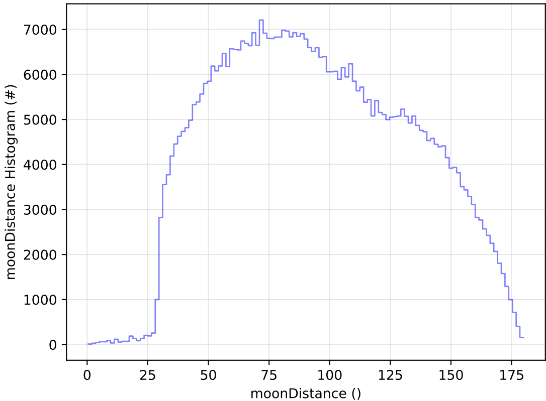
too_elab_r256_d3_griz_v3.4_10yrs All sky i band: moonDistance Histogram
