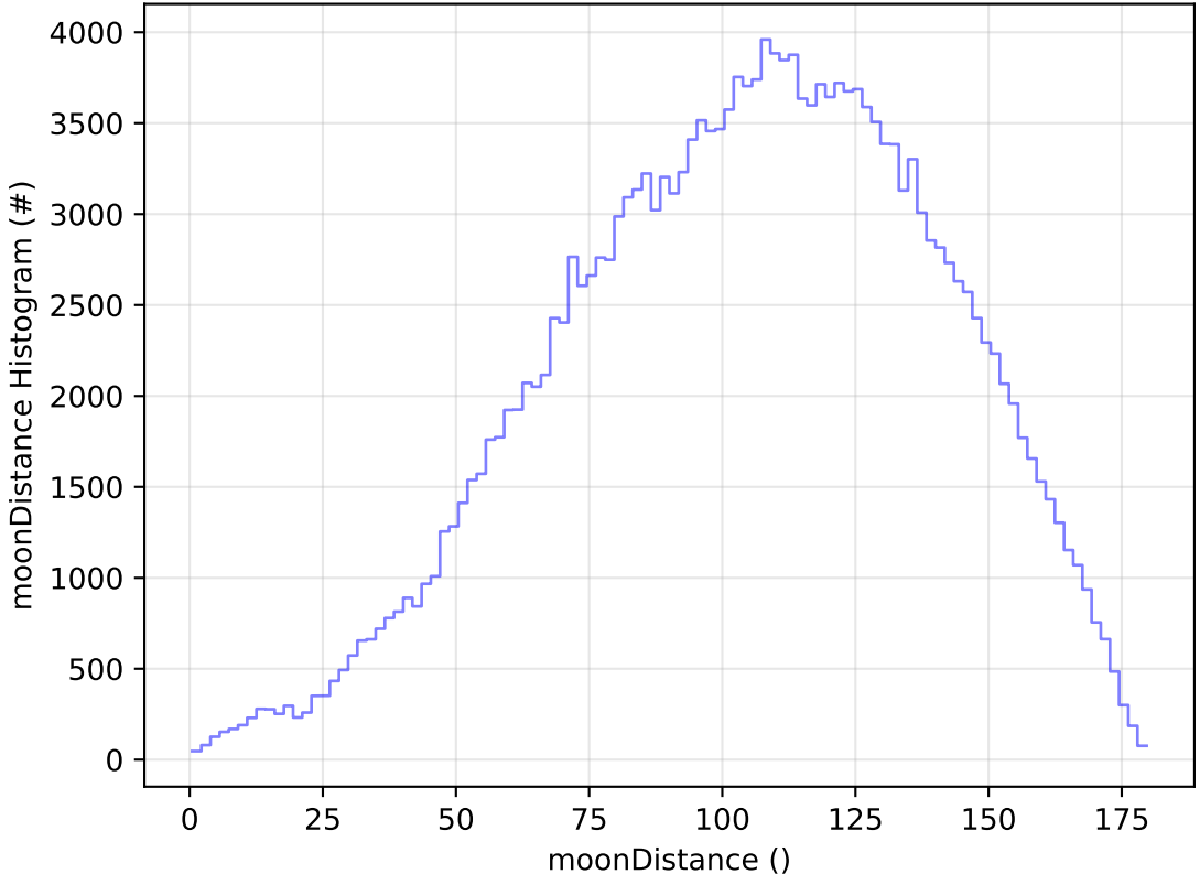
too_elab_r256_d3_griz_v3.4_10yrs All sky g band: moonDistance Histogram
