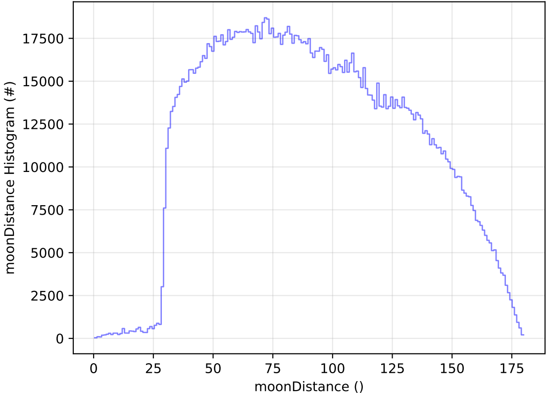
too_elab_r256_d3_griz_v3.4_10yrs All sky all bands: moonDistance Histogram
