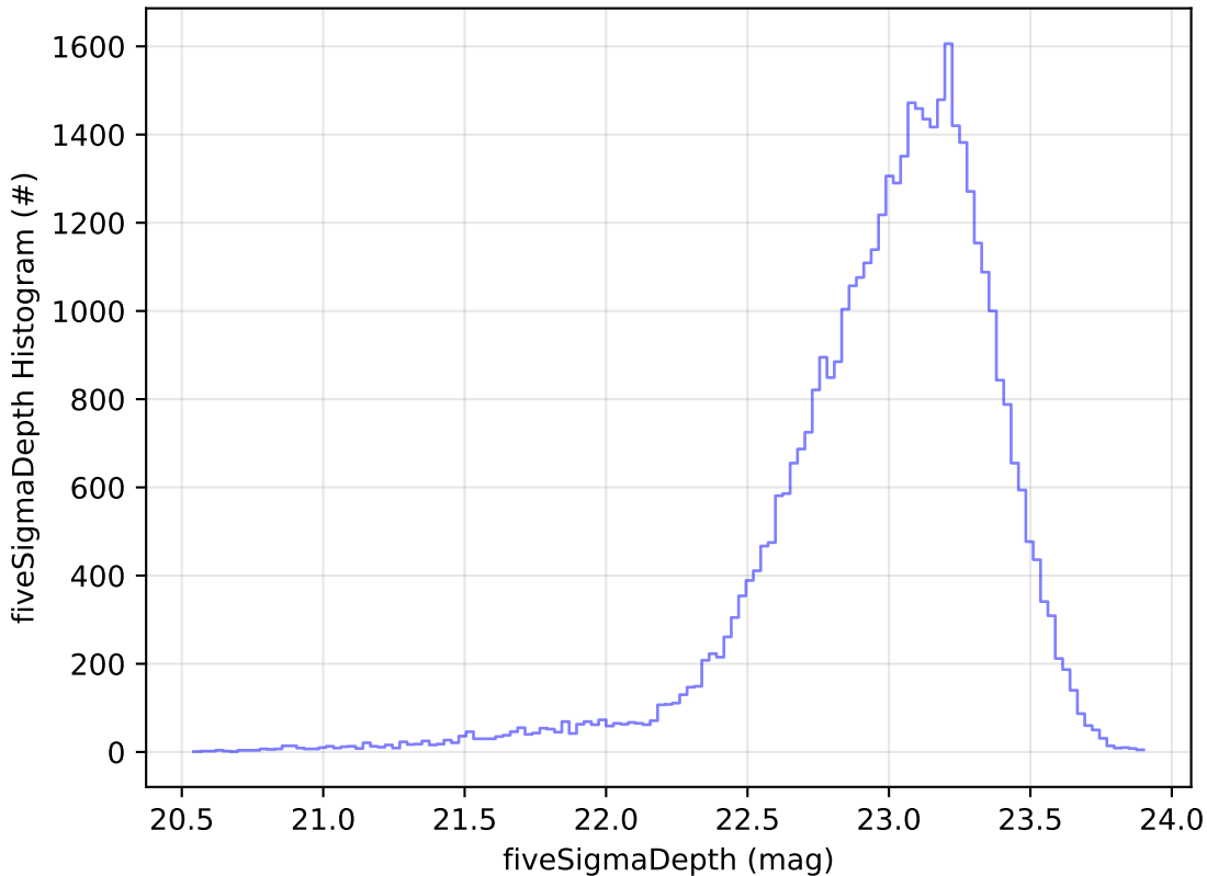
too_elab_r256_d3_griz_v3.4_10yrs Yr 1 z band: fiveSigmaDepth Histogram
