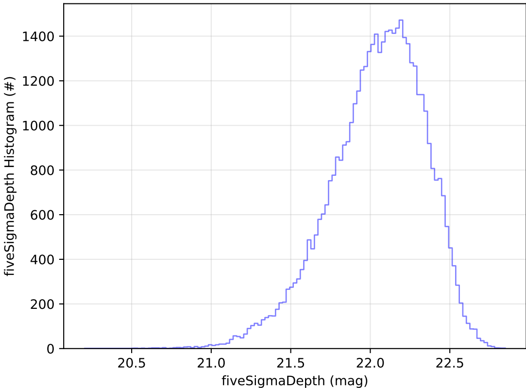
too_elab_r256_d3_griz_v3.4_10yrs Yr 1 y band: fiveSigmaDepth Histogram
