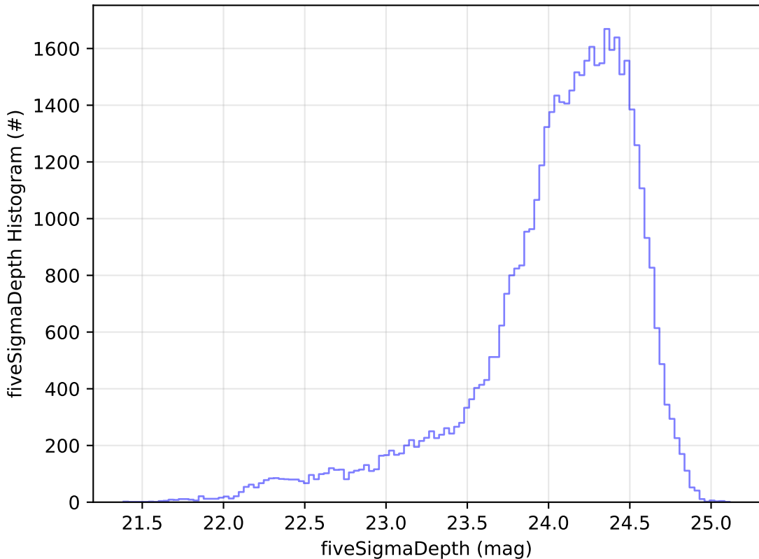
too_elab_r256_d3_griz_v3.4_10yrs Yr 1 r band: fiveSigmaDepth Histogram
