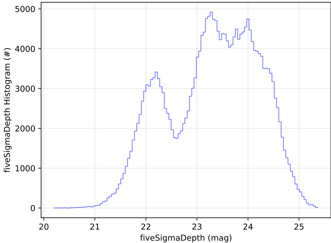
too_elab_r256_d3_griz_v3.4_10yrs Yr 1 all bands: fiveSigmaDepth Histogram
