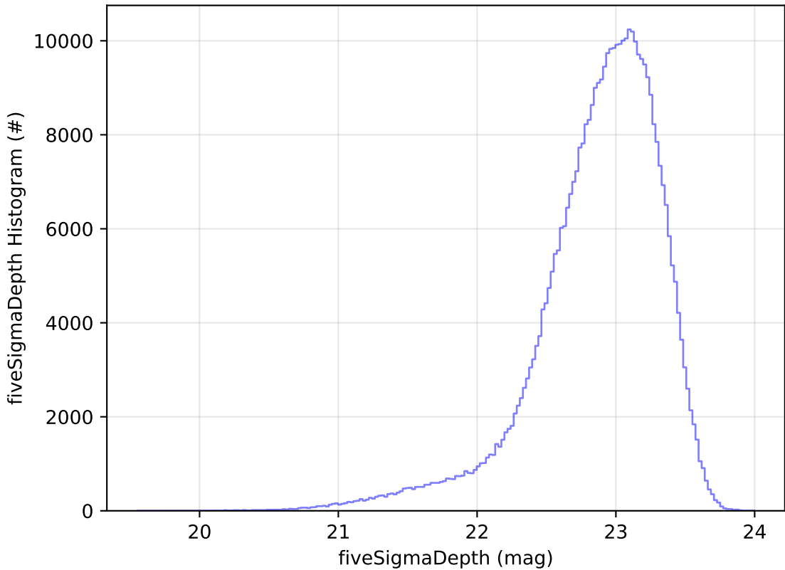
too_elab_r256_d3_griz_v3.4_10yrs WFD z band: fiveSigmaDepth Histogram
