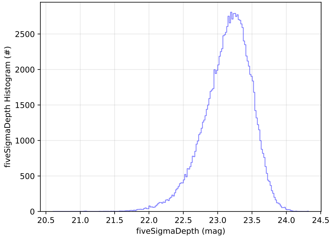
too_elab_r256_d3_griz_v3.4_10yrs WFD u band: fiveSigmaDepth Histogram
