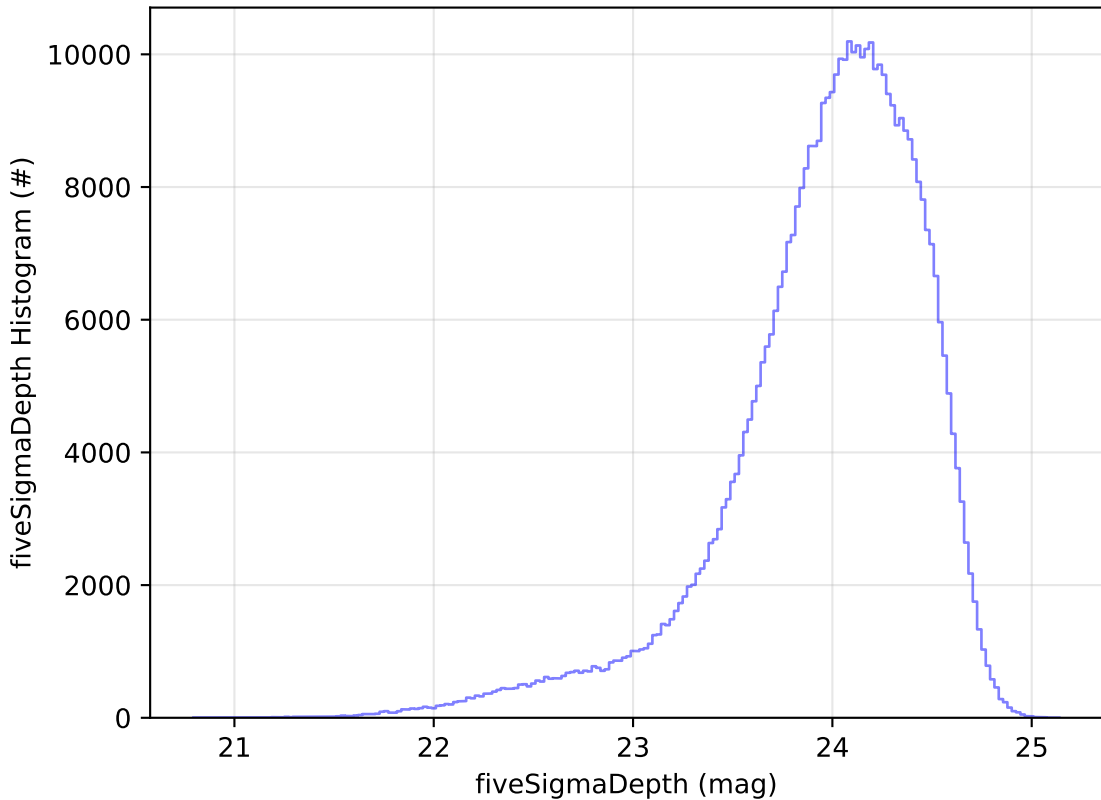
too_elab_r256_d3_griz_v3.4_10yrs WFD r band: fiveSigmaDepth Histogram
