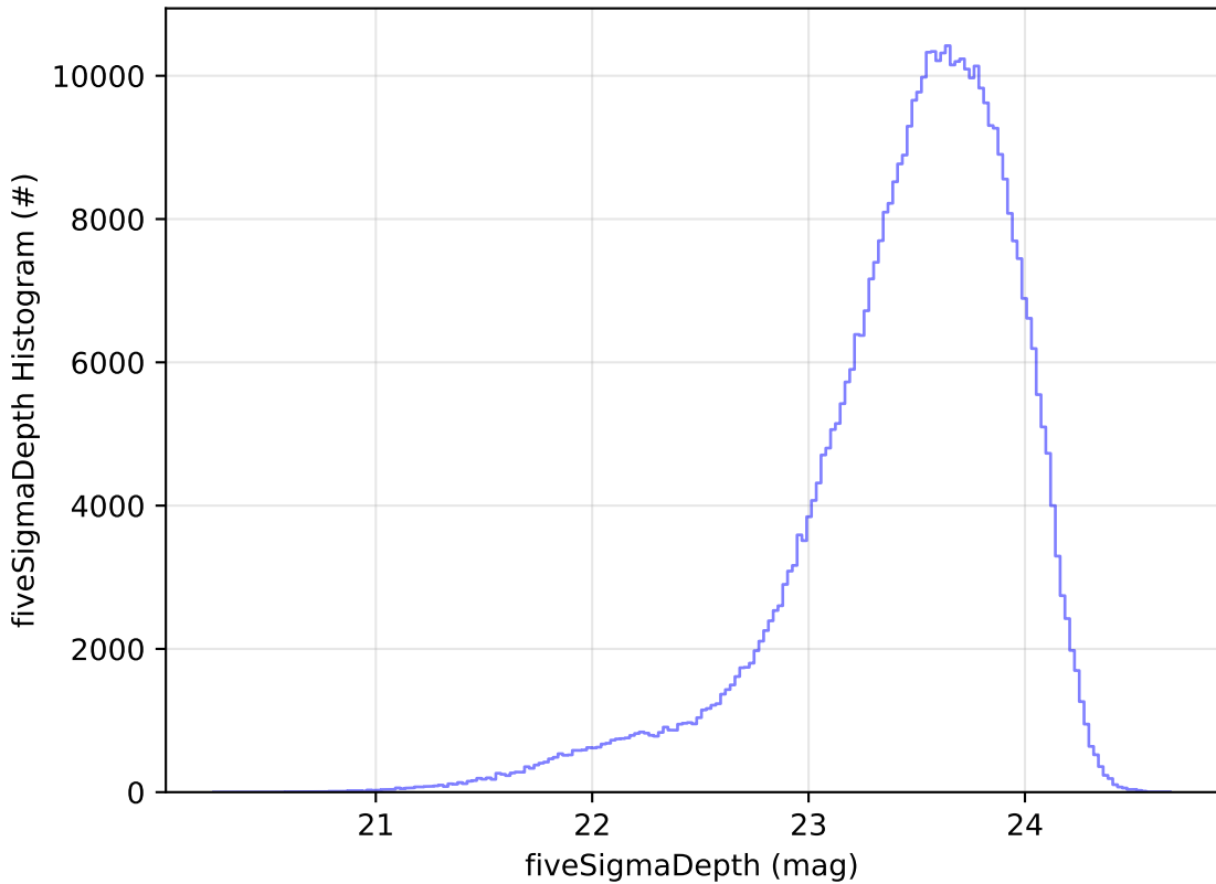
too_elab_r256_d3_griz_v3.4_10yrs WFD i band: fiveSigmaDepth Histogram
