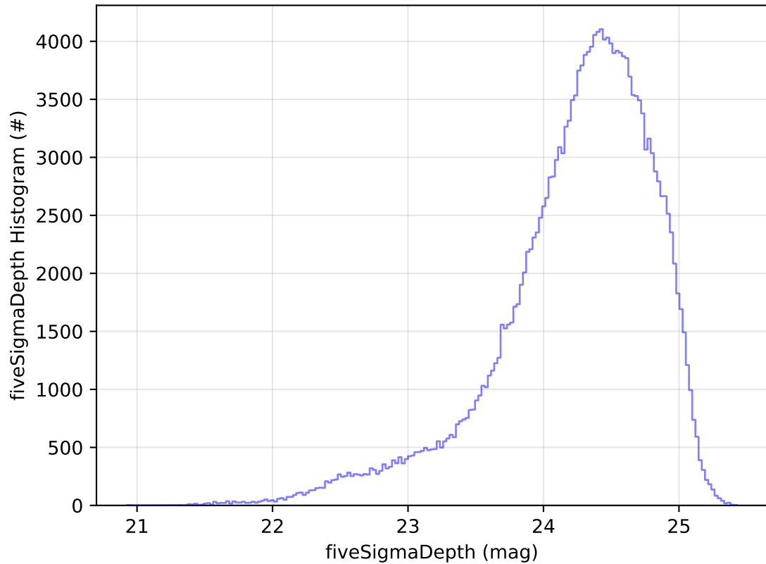
too_elab_r256_d3_griz_v3.4_10yrs WFD g band: fiveSigmaDepth Histogram
